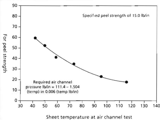
Figure 1. Relationship between the air-channel pressure required to verify a specified field peel strength of 2.6 N/mm and 15.0 lb./in. at various sheet temperatures, from Stark et al. (2004).
