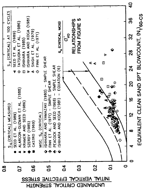
FIG. 11. Comparison of Undrained Critical Strength Ratios from Field Performance and Laboratory Shear Tests
