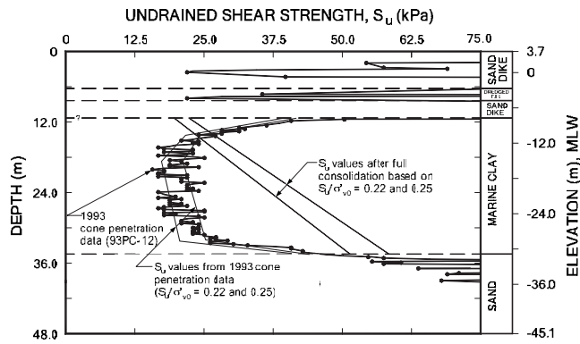
Fig. 3. Undrained shear strength profile below Craney Island west perimeter dike in 1993
