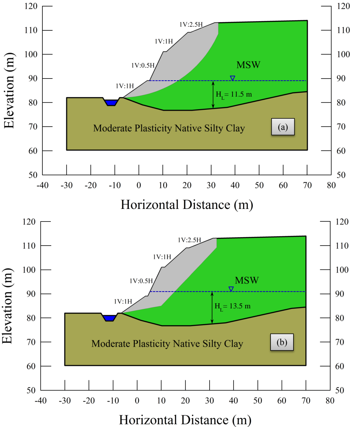
Figure 11. Cross- sections showing location of (a) circular and (b) planar failure surfaces.
