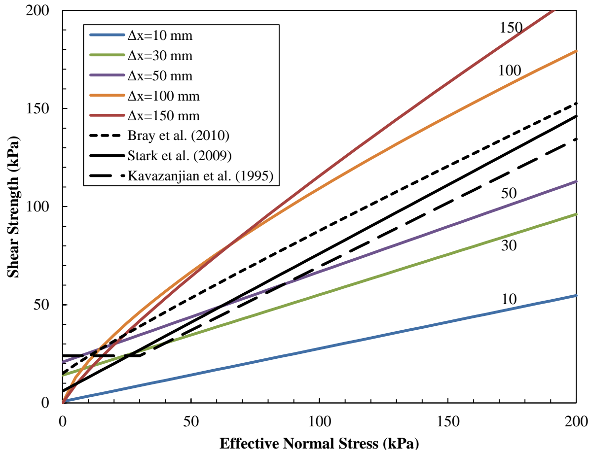
Figure 10. MSW shear strength envelopes.
