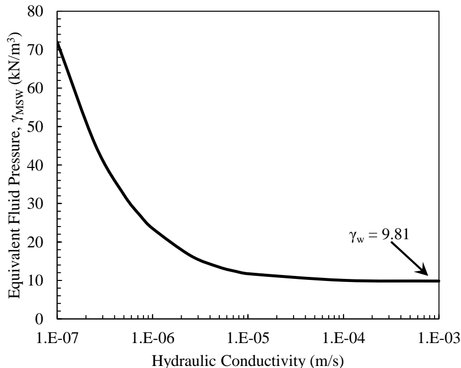
Figure 12. Dependence of equivalent fluid unit weight, \gamma_{\text{fluid, equivalent}} on MSW saturated hydraulic conductivity, K_{\text{waste, sat}}
