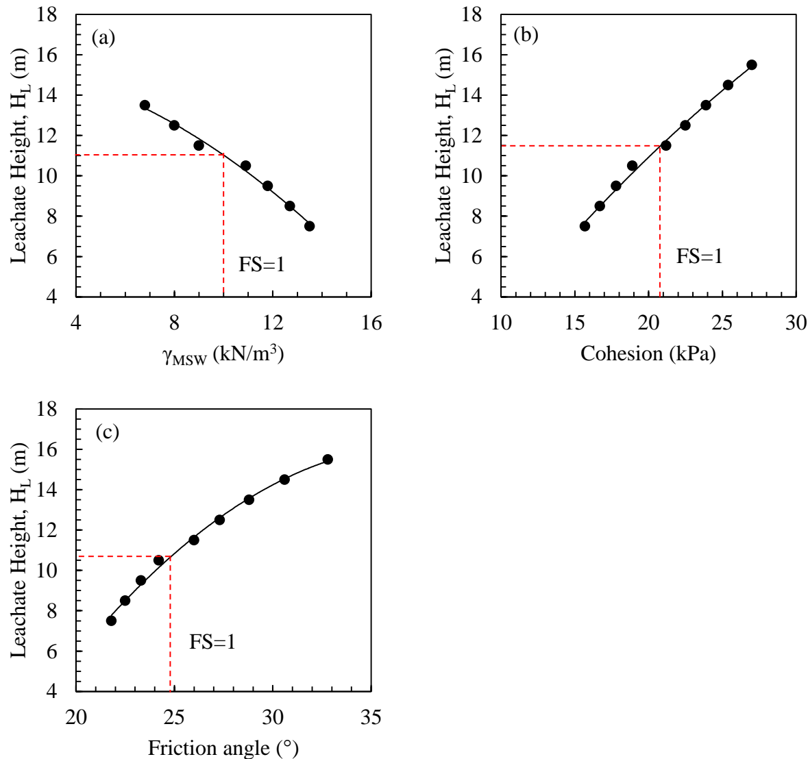
Figure 14. Sensitivity of Inverse analysis to MSW input parameters for FS of unity.
